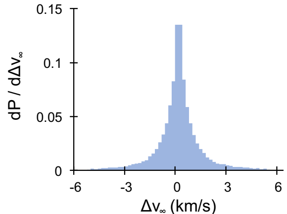
Fig. 1. Distribution of the gravitational \Delta v_\infty for random encounter geometries between Earth and LPCs marginally bound to the Sun near the Earth’s surface.
