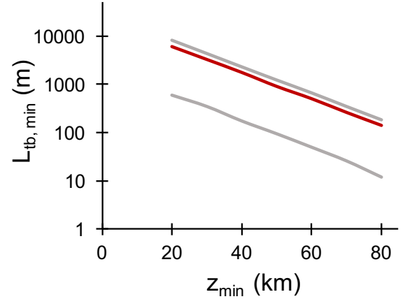
Fig. 2. Minimum diameter of transporting body to guarantee total expansion of < 10\% as a function of minimum encounter altitude. The red line indicates the result for an encounter velocity of 42 \text{ km s}^{-1} , and the gray lines represent the upper and lower bounds, corresponding to the maximum and minimum encounter velocities of 72 \text{ km s}^{-1} and 12 \text{ km s}^{-1} , respectively.
