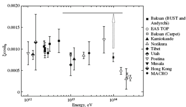
Figure 3. Summary of world data on GCR anisotropy. Presented results are converted to the equator (projection \xi \cos \delta_0 of the anisotropy vector onto the equator plane). The horizontal bar shows approximate level of the true anisotropy after correction by the cosine of declination \delta_0 determined in the present paper.
