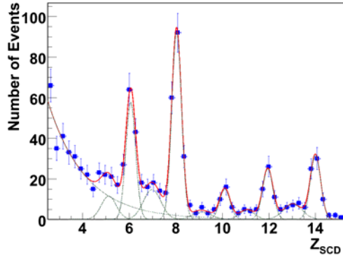
Figure 2: Subset of charge distribution using the average of signals from the top and bottom SCD layers after event selection and consistency requirements. The distribution is fitted with a multi-Gaussian function with exponential function.
