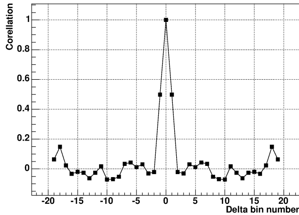
Figure 1. The mean correlation function of carbon.
