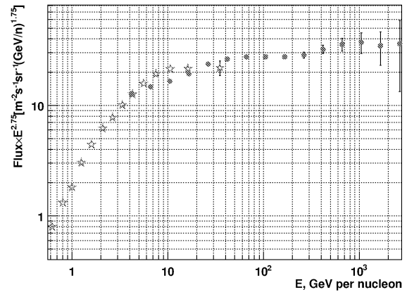
Figure 3. Spectrum of carbon. Full circles: present work, open stars: HEAO-3-C2 [2].
