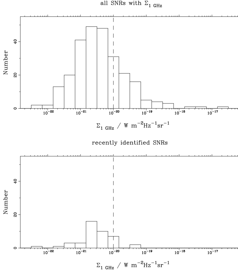
Figure 1. Histograms in surface brightness at 1 GHz for (top) all 258 Galactic SNRs with 1-GHz flux densities, and (bottom) the remnants included in the catalogue since 2004. The dashed lines mark the nominal completeness limit of the catalogue, see text.
